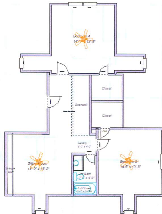
Upstairs floor plan
